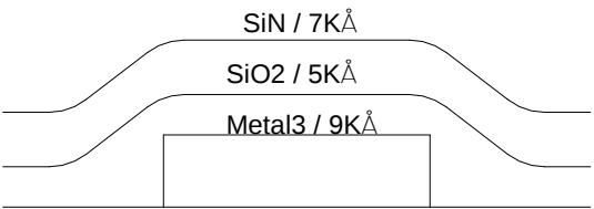
FOR PROCESS CROSS-SECTION
