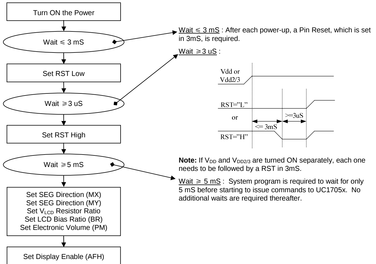
Figure 8: Reference Power-Up Sequence
