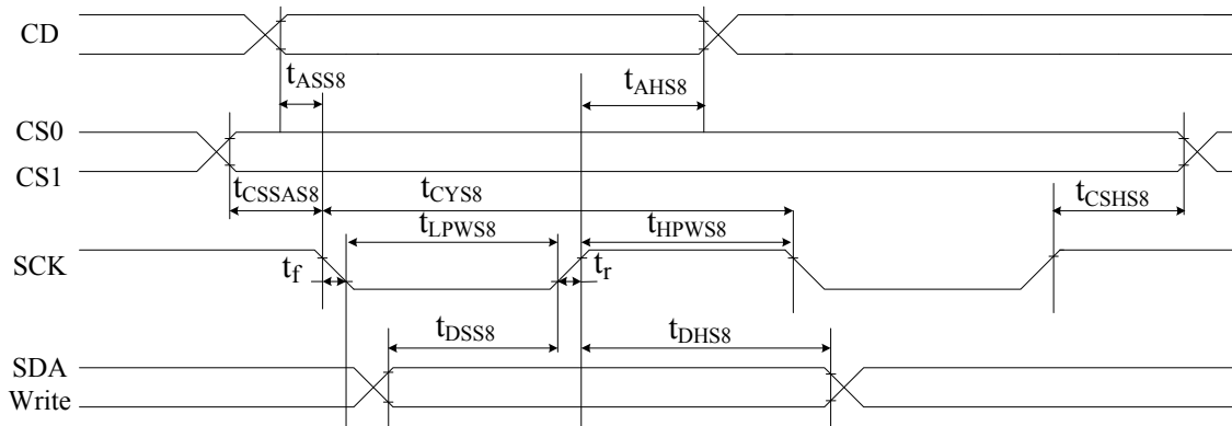
FIGURE 14: Serial Bus Timing Characteristics (for S8)
