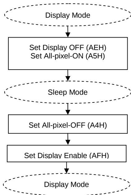
FIGURE 10: Reference Enter/Exit Sleep Mode Sequence
